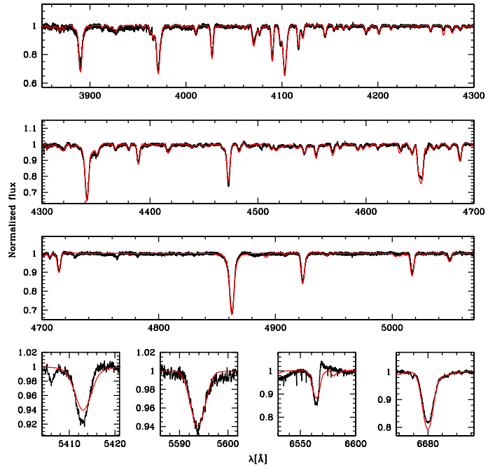
Fig. A.3. Best fit (red) of the observed spectrum (black) of HD 154811.
