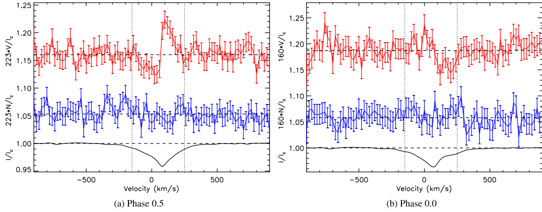
Figure 8. Left: LSD profile at phase 0.5, Stokes V: definite detection (FAP = 9\text{e}-7 per cent), \langle B_z \rangle = -290 \pm 95 G. Diagnostic null N: ND (FAP = 72 per cent), \langle N_z \rangle = -2 \pm 95 G. Right: LSD profile at phase 0.0, Stokes V: no detection (FAP = 2 per cent), \langle B_z \rangle = +335 \pm 200 G. Diagnostic null N: ND (FAP = 91 per cent), \langle N_z \rangle = -71 \pm 199 G.
